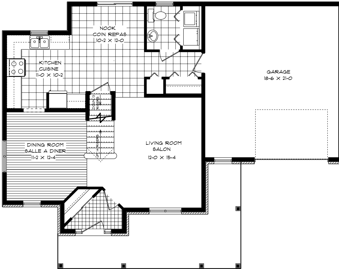
MAIN FLOOR PLAN PLANCHER PRINCIPAL
