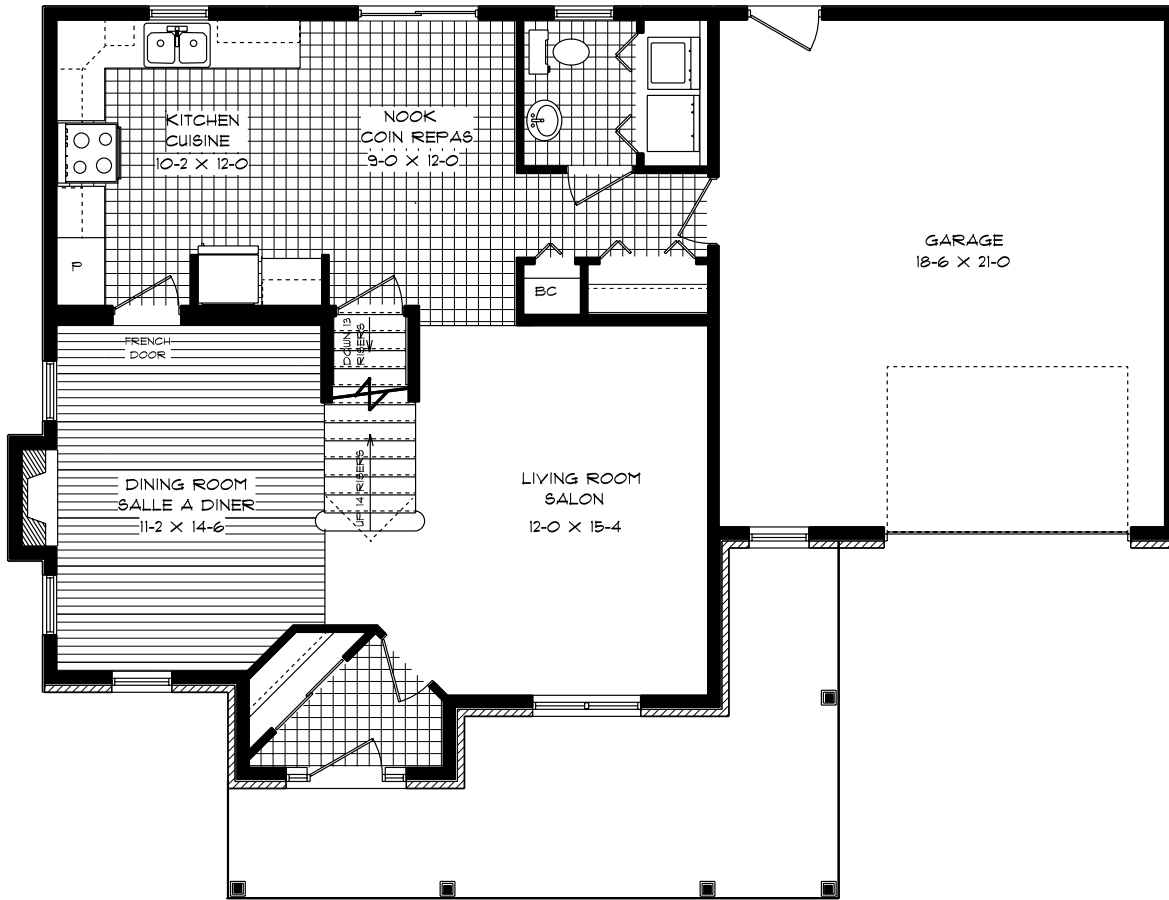
MAIN FLOOR PLAN PLANCHER PRINCIPAL
